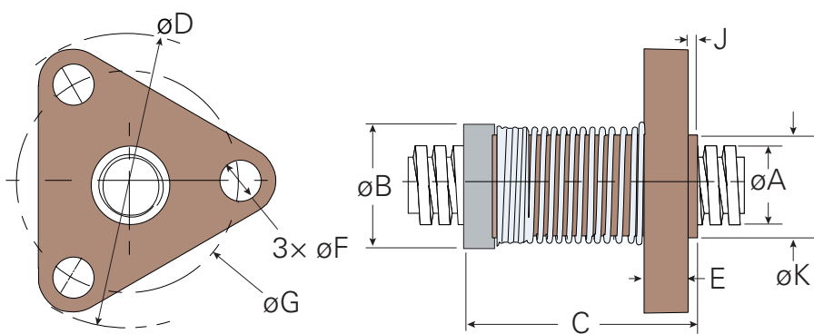
Triangular Flange
