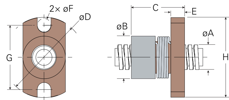
Rectangular Flange
