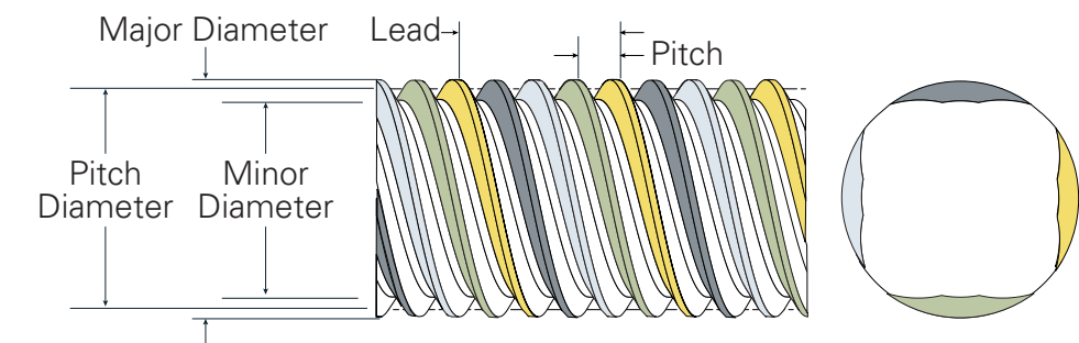
Four Start
