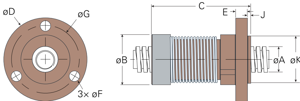
Round Flange
