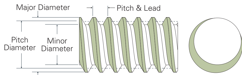
Single Start
