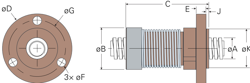
Round Flange
