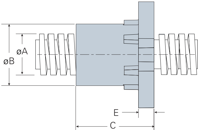
Three-Hole Flange Diameter Ranges:. 195 – 1.000 in 5.5 – 25.4 mm
