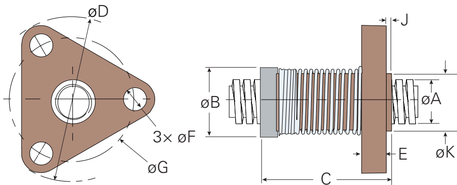
Triangular Flange
