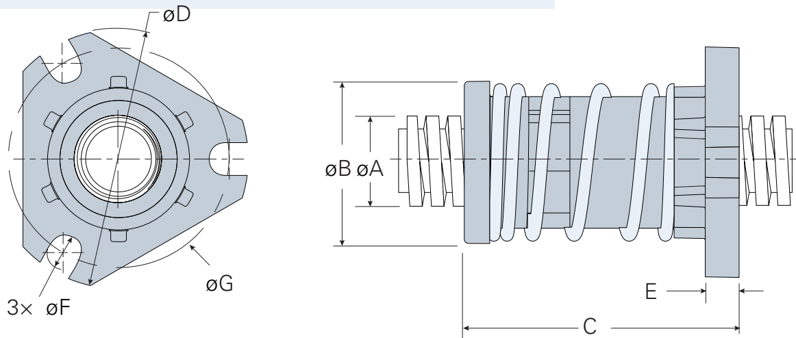
Three-Hole Flange Diameter Ranges: .195 – 1.000 in 5.5 – 25.4 mm
