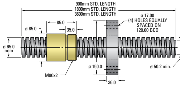
65mm Trapezoidal Thread Lead Accuracy \pm 6.25 \mu\text{m}/25\text{mm}
