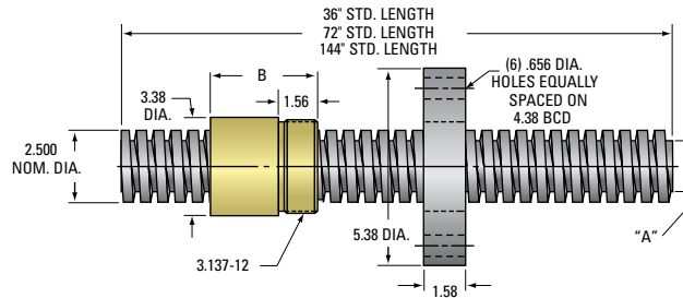
2½" ACME THREAD Lead Accuracy 0.0003 in/in
