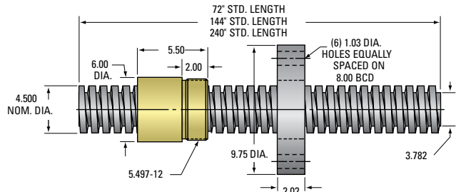
4½" ACME THREAD Lead Accuracy 0.0006 in/in
