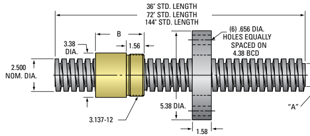
2½" ACME THREAD Lead Accuracy 0.0003 in/in
