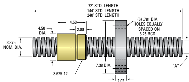
3/8" ACME THREAD Lead Accuracy 0.0006 in/in
